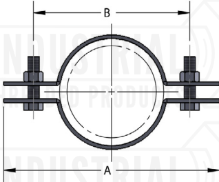
FIG. 49PC RISER CLAMP FOR PLASTIC PIPE, PLASTIC COATED
