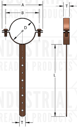
FIG. 131CT MILFORD HANGER, COPPER TUBE SIZE
