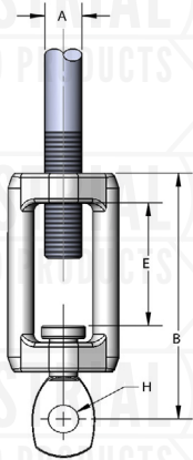
FIG. 114 TURNBUCKLE ADJUSTER
